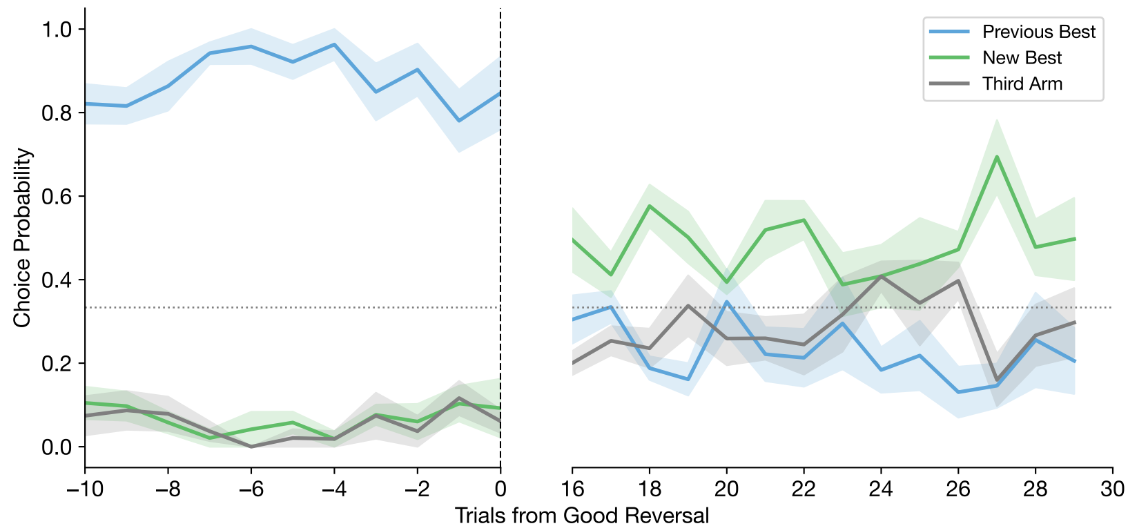
Good Reversal-Aligned Choices (mean \pm se across subjects | n=6 subjects, n=50 reversals) (Skipping first 15 trials post-reversal)
